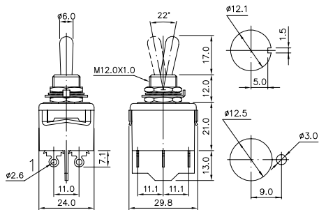
PANEL LAYOUT
